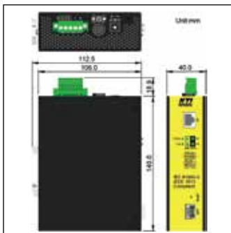
DIN-Rail Dimension
